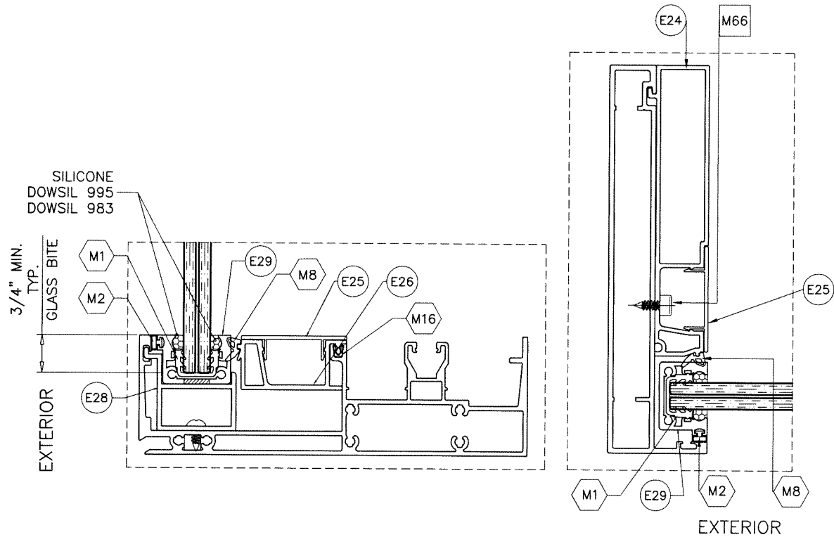
GLAZING DETAIL AT FIXED PANEL 9/16" LAM. GLASS
