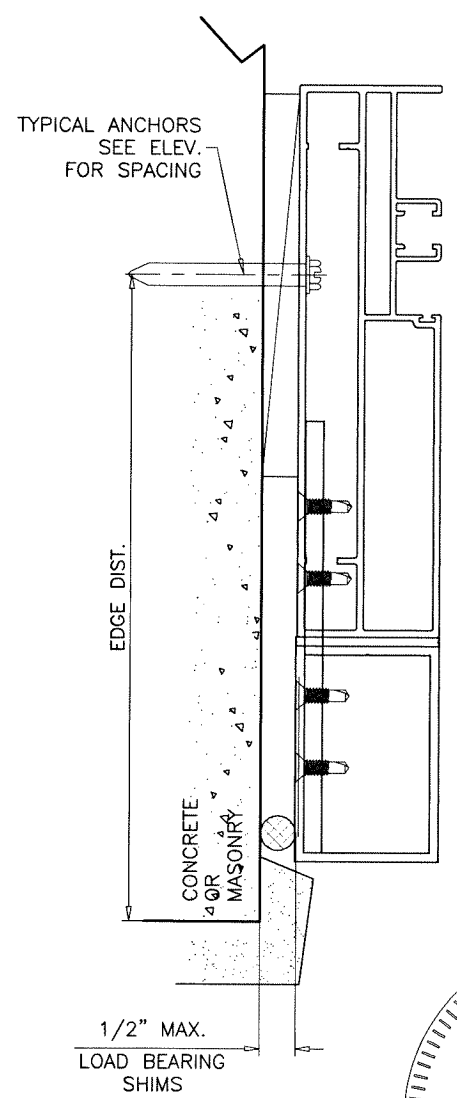
3 TRACK FRAMES ANCHOR LOCATIONS
