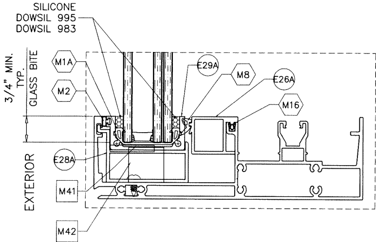
GLAZING DETAIL AT FIXED PANEL 1-7/16" OVERALL INSUL. LAM. GLASS
