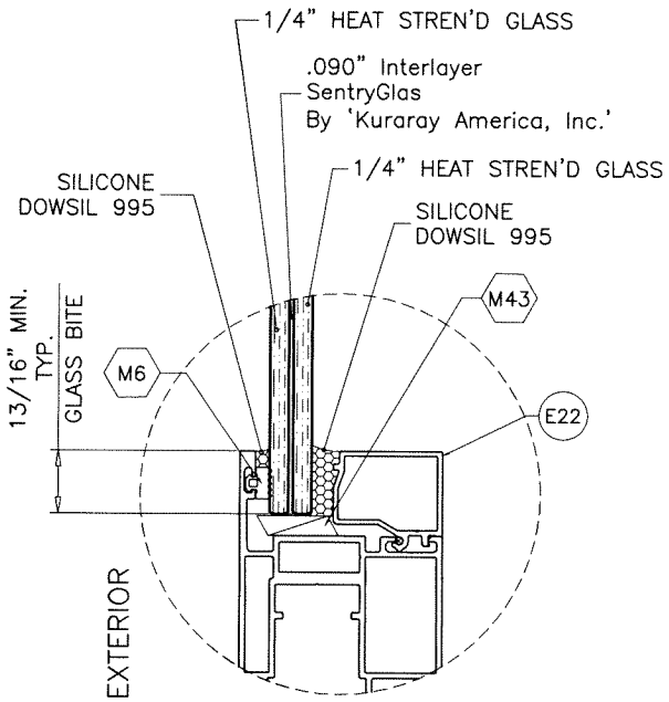
GLASS TYPE 'A' 9/16" LAM. GLASS GLAZING DETAIL AT MOVING PANEL
