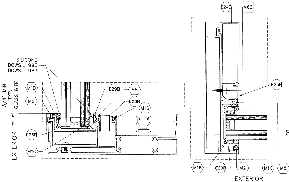
GLAZING DETAIL AT FIXED PANEL 1-1/2" OVERALL INSUL. DOUBLE LAM. GLASS
